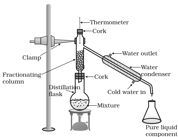
Fig. 2.10: Fractional distillation
