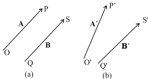
Fig. 4.2 (a) Two equal vectors \mathbf{A} and \mathbf{B} . (b) Two vectors \mathbf{A}' and \mathbf{B}' are unequal though they are of the same length.
